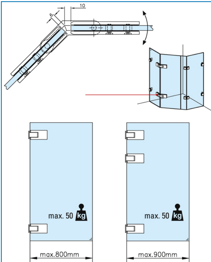
Türscharnier
