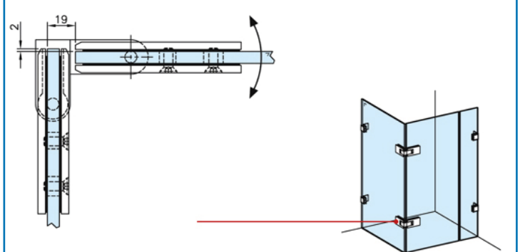
Türscharnier
