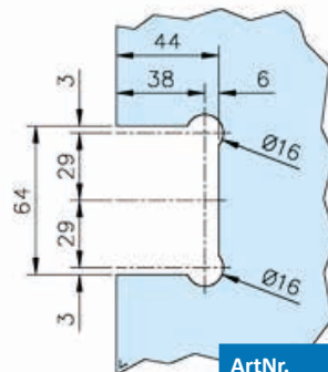
Glas/Glas Montage
